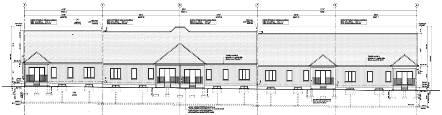
REAR ELEVATION
